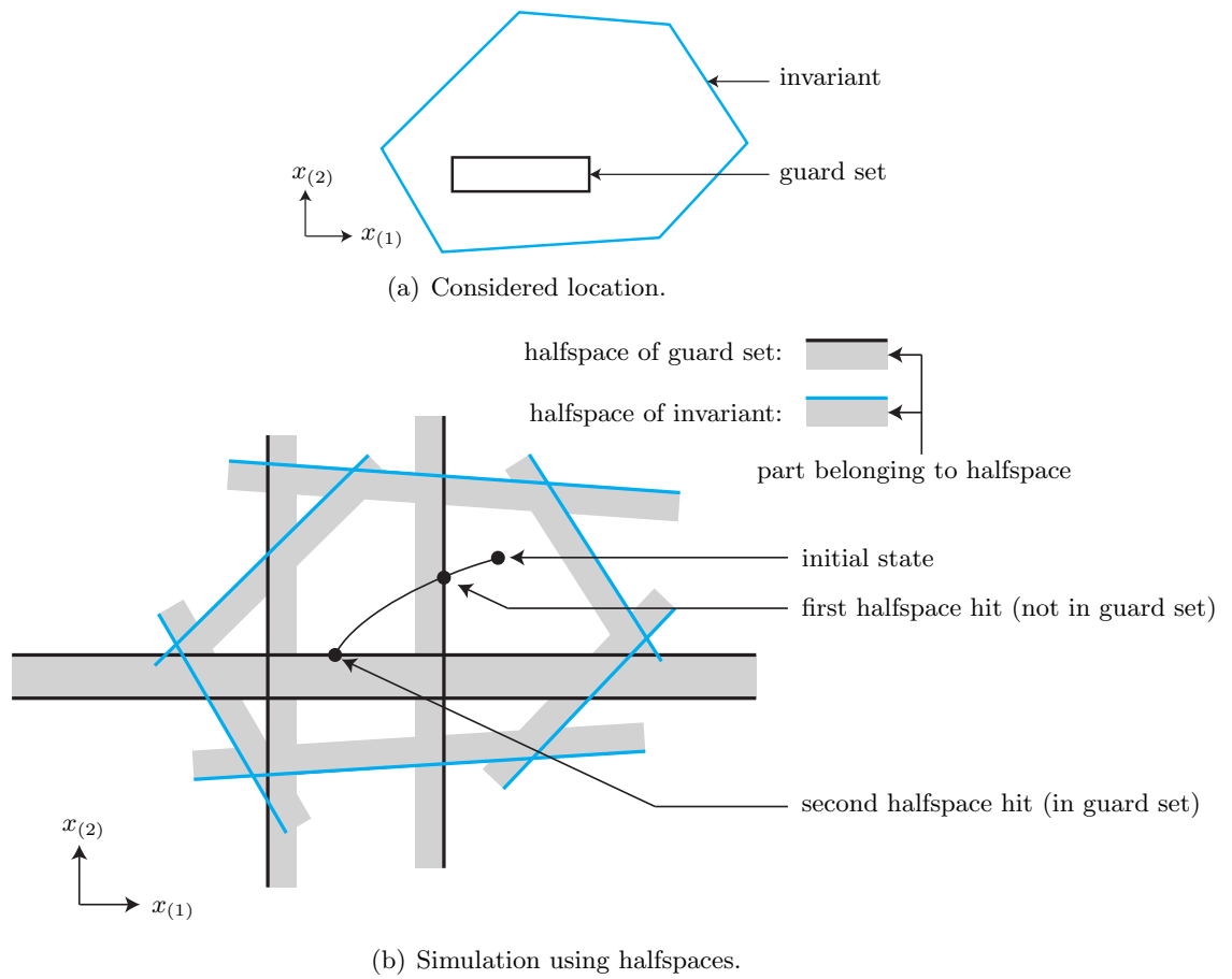
Figure 54: Illustration of the algorithm for simulating a hybrid automaton.
