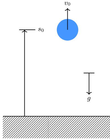
Figure 51: Example for a hybrid system: bouncing ball.
