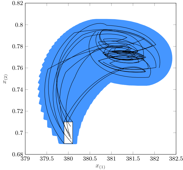
Figure 50: Illustration of the reachable set of nonlinear differential-algebraic example. The white box shows the initial set and the black lines show simulated trajectories.
