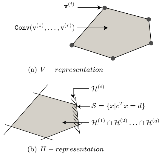
Figure 3: Possible representations of a polytope.
