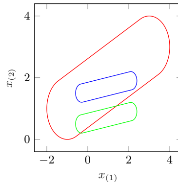
Figure 34: Capsules generated in lines 6, 10, and 14 of the capsule example in Sec. 10.1.7.
