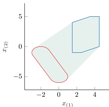
Figure 38: Sets generated in lines 21-25 of the spectrahedral shadow example in Sec. 10.1.10.
