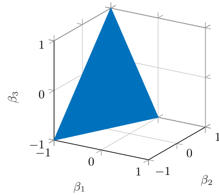
Figure 37: Visualization of the constraints for the conZonotope object generated in the constrained zonotope example in Sec. 10.1.9.
