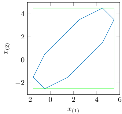
Figure 26: Sets generated in lines 18-19 of the zonotope example in Sec. 10.1.1.
