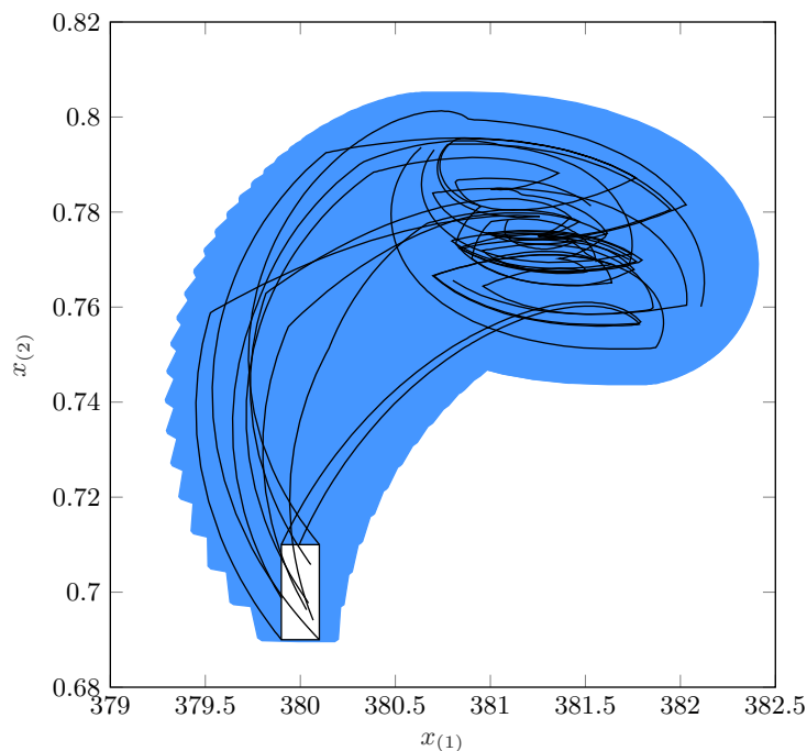
Figure 49: Illustration of the reachable set of nonlinear differential-algebraic example. The white box shows the initial set and the black lines show simulated trajectories.
