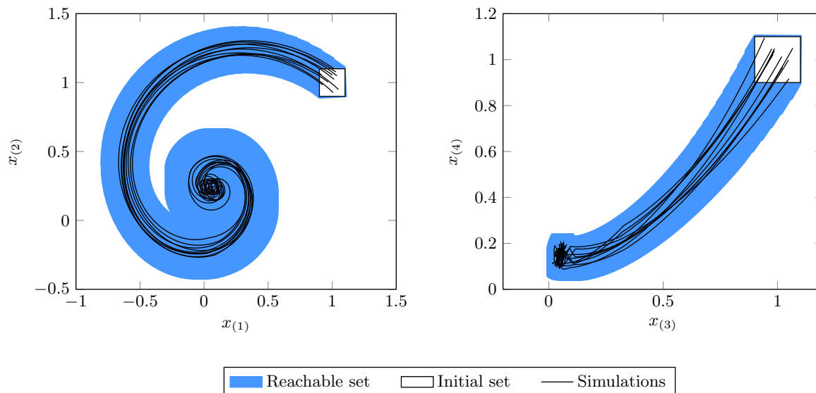
Figure 40: Illustration of the reachable set of the linear example. The white box shows the initial set and the black lines show simulated trajectories.
