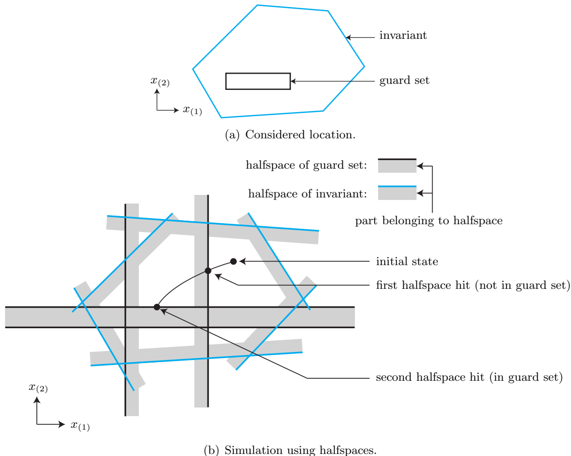
Figure 53: Illustration of the algorithm for simulating a hybrid automaton.
