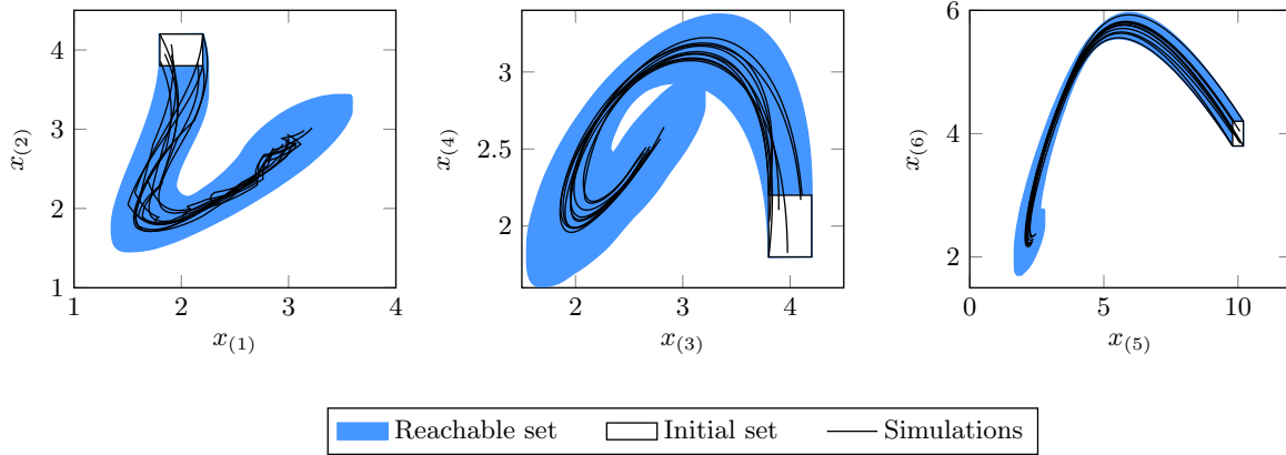
Figure 43: Illustration of the reachable set of the linear example. The white box shows the initial set and the black lines show simulated trajectories.
