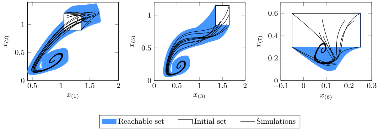
Figure 45: Illustration of the reachable set of the seven-dimensional example for non-convex set representation. The white box shows the initial set and the black lines show simulated trajectories.
