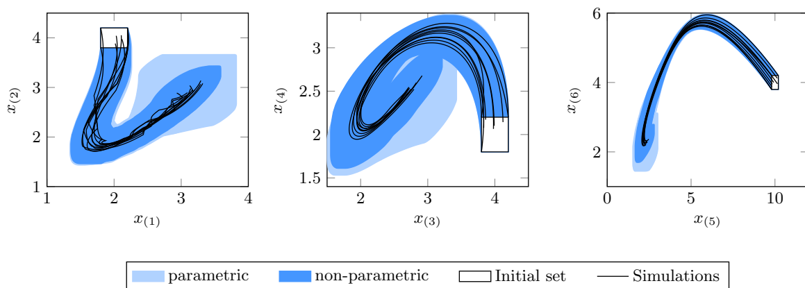
Figure 47: Illustration of the reachable set of the nonlinear parametric example. The light-blue region shows the reachable set with uncertain parameters, while the blue area shows the reachable set without uncertain parameters. The white box shows the initial set and the black lines show simulated trajectories.
