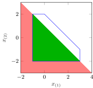
Figure 37: Intersection (green) between the halfspace (red) and the polytope (blue) generated by the example in Sec. 9.1.11.
