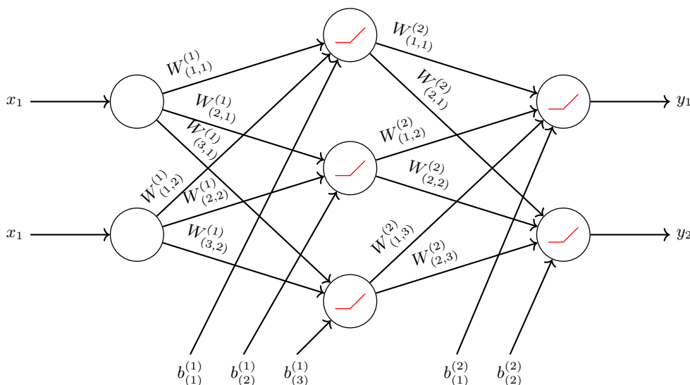
Figure 19: Feed-forward neural network with N = 2 layers.
