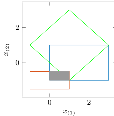
Figure 25: Sets generated in lines 11-14 of the interval example in Sec. 9.1.2.
