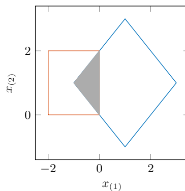
Figure 33: Sets generated in lines 7-9 of the zonotope bundle example in Sec. 9.1.8.
