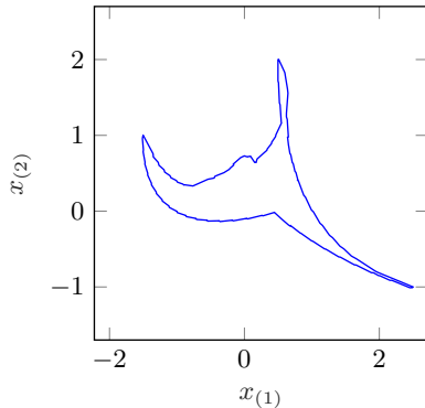
Figure 30: Constrained polynomial zonotope generated in lines 21-28 of the constrained polynomial zonotope example in Sec. 9.1.6
