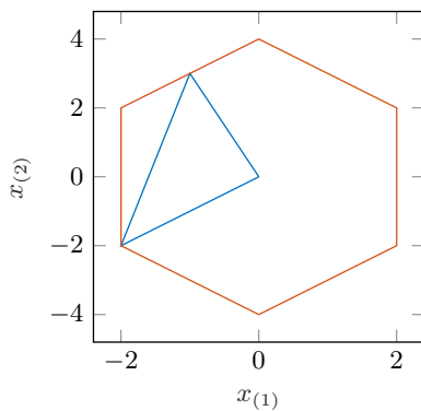
Figure 34: Zonotope (red) and the corresponding constrained zonotope (blue) generated in the constrained zonotope example in Sec. 9.1.9
