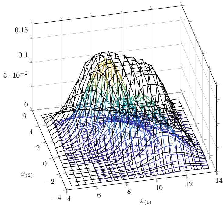
Figure 36: Sets generated in lines 10-15 of the probabilistic zonotope example in Sec. 9.1.10.
