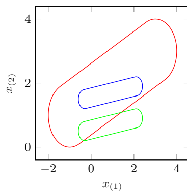
Figure 32: Capsules generated in lines 6, 10, and 14 of the capsule example in Sec. 9.1.7.
