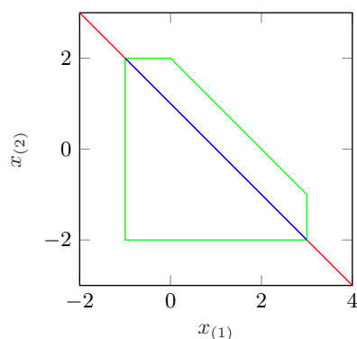
Figure 38: Constrained hyperplane generated by the example code in Sec. 9.1.12.
