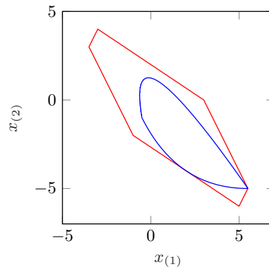
Figure 29: Quadratic map calculated with zonotopes (red) and polynomial zonotopes (blue).
