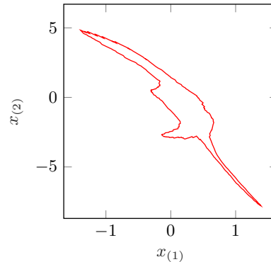
Figure 31: Quadratic map computed in lines 31-34 of the constrained polynomial zonotope example in Sec. 9.1.6.
