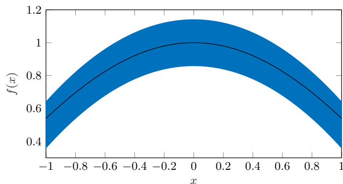
Figure 8: Function f(x) = \cos(x) (black) and the enclosing Taylor model \mathcal{T}(x) in (21) (blue).
