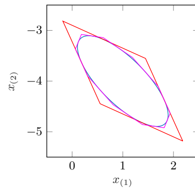
Figure 27: Sets generated in lines 22-24 of the ellipsoid example in Sec. 9.1.3.
