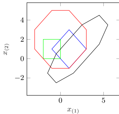
Figure 23: Zonotopes generated in lines 9-12 of the zonotope example in Sec. 9.1.1.
