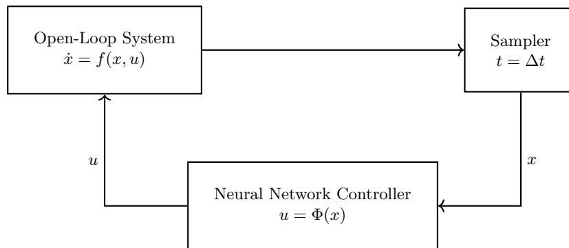
Figure 11: Structure of a neural network controlled system.
