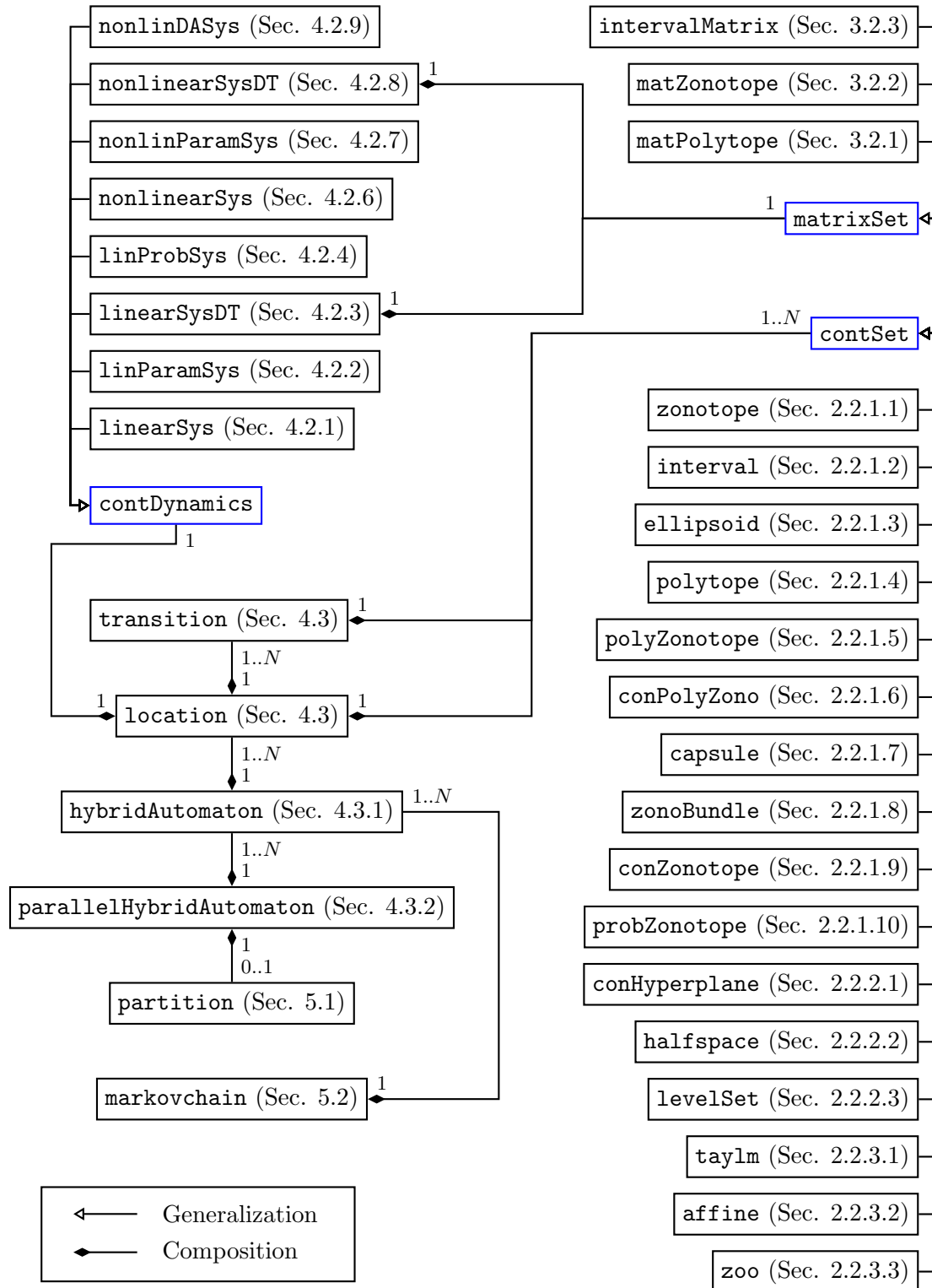
Figure 1: Unified Modeling Language (UML) class diagram of CORA.
