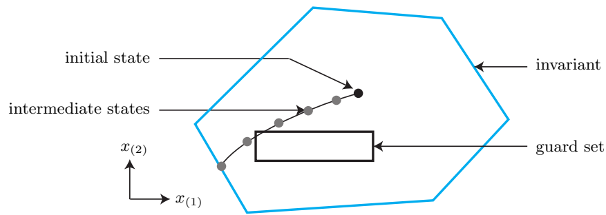
Figure 54: Guard intersections can be missed when one only checks whether intermediate states are in any guard set.
