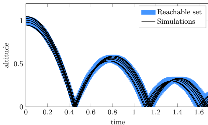
Figure 51: Illustration of the reachable set of the bouncing ball.
