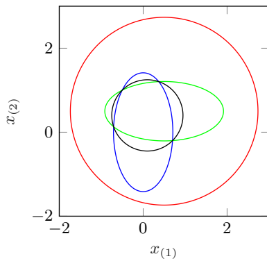
Figure 26: Ellipsoids generated in lines 12-15 of the ellipsoid example in Sec. 9.1.3.
