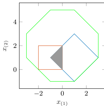
Figure 28: Sets generated in lines 13-16 of the polytope example in Sec. 9.1.4.
