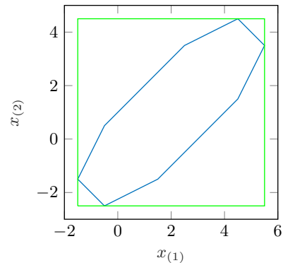
Figure 24: Sets generated in lines 18-19 of the zonotope example in Sec. 9.1.1.
